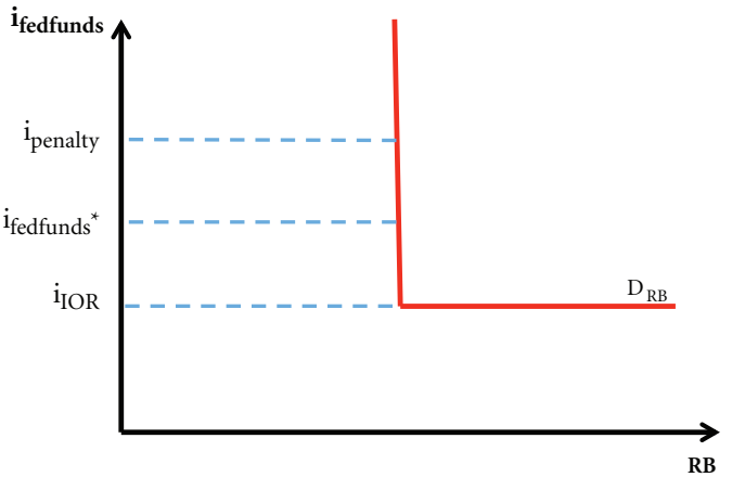
Figure C.1 Demand for Reserve Balances in the Federal Funds Market
